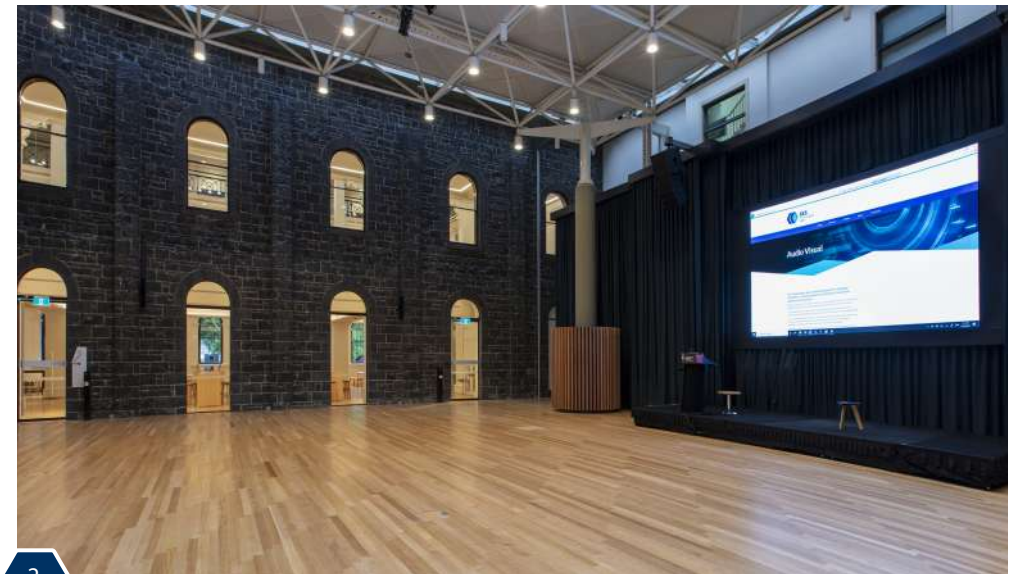
2 Function Space
